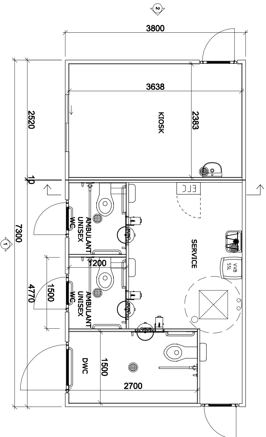
PLAN
